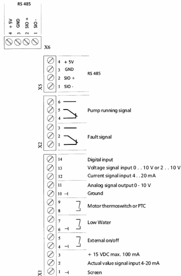
Fig. 6 Connection overview
