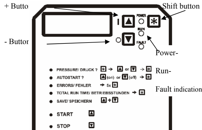
Fig. 3 Operating panel
