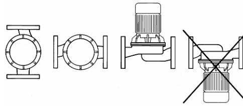
Fig. 1 Pump Installation
