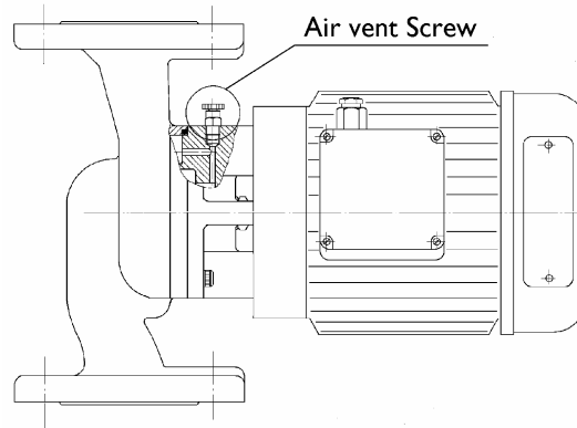
Fig. 2 Air venting
