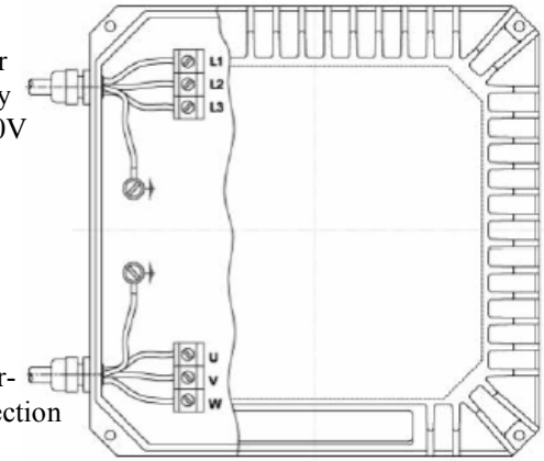
Fig. 4 Installation overview for HV 3.15 – 3.22
